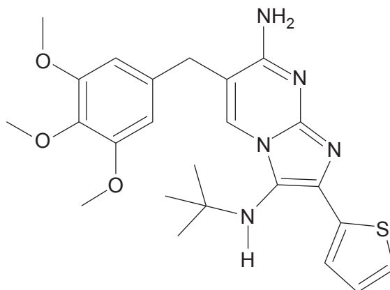
Compound X
