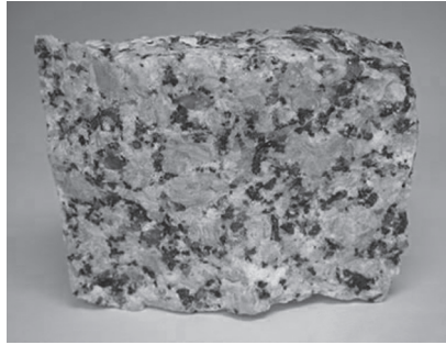
© Geology.com
